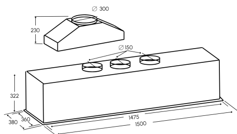
Cut-out Dimensions* W1475 x D265mm
