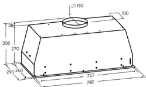
Cut-out Dimensions W765 x D270mm
