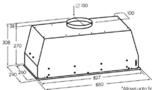
Cut-out Dimensions W835 x D270mm
